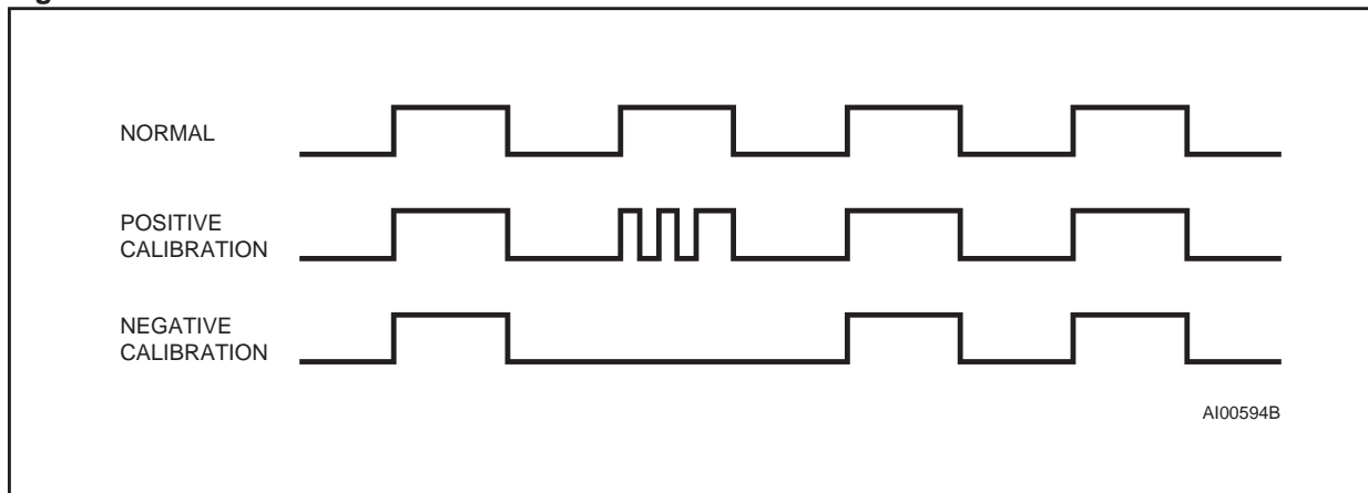
Figure 10. Calibration Waveform
