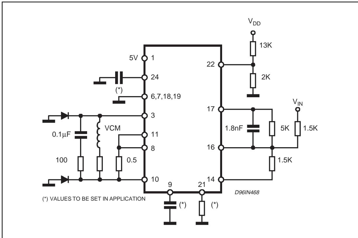
Figure 1: Application Circuit
