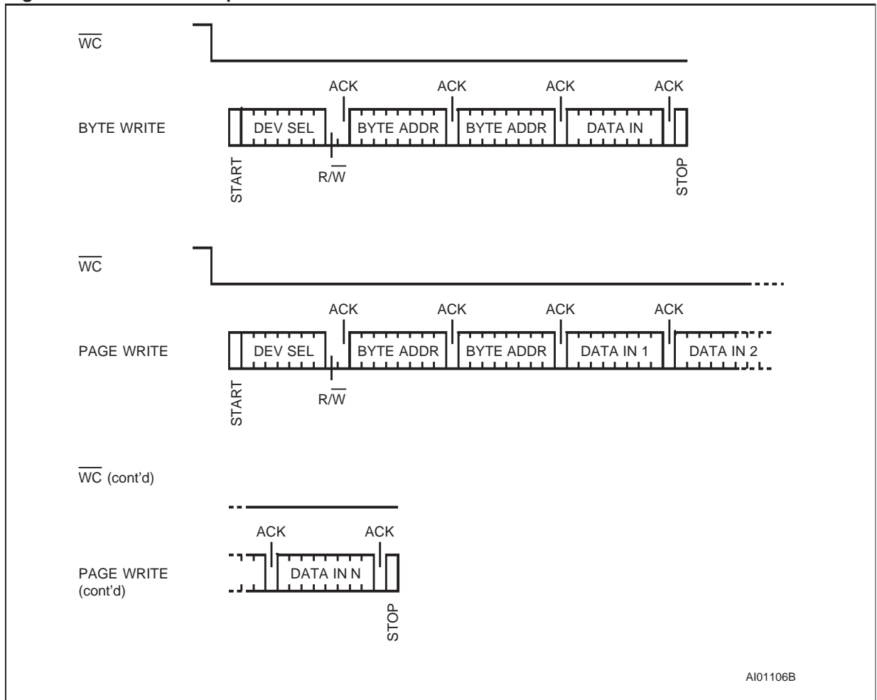
Figure 7. Write Mode Sequences with \overline{WC}=0
