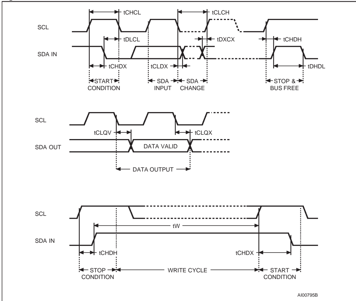
Figure 10. AC Waveforms
