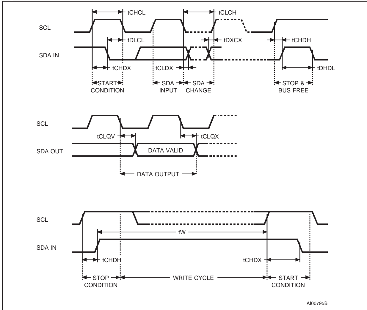
Figure 9. AC Waveforms
