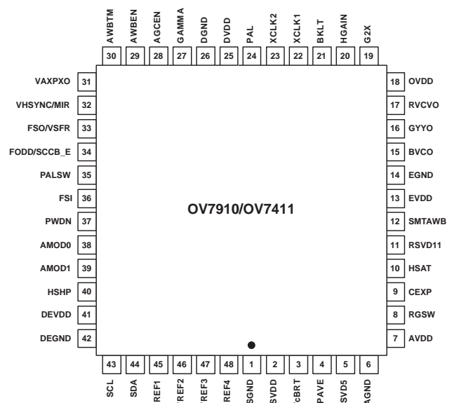
Figure 1 OV7910/OV7411 Pin Diagram
