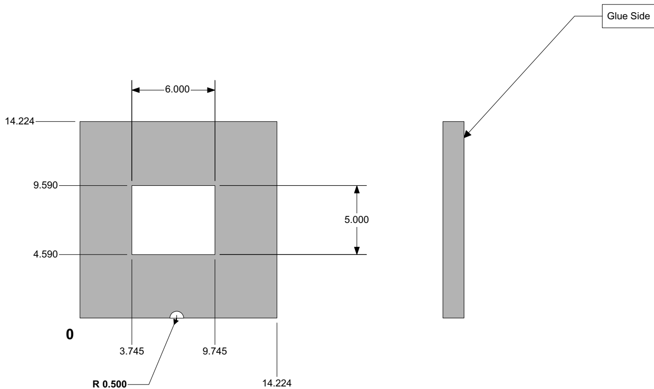
Figure 9 OV7910/OV7411 Mask Drawing
