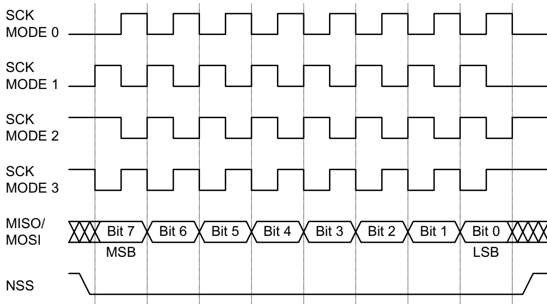
Figure 3. Timing For Mode 0 and Mode 3
