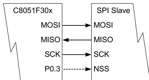
Figure 1. Hardware Configuration
