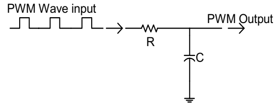
Figure 1. Low-Pass Filter
