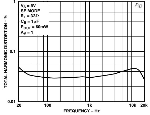
Figure 5. SE Out THD + N vs. Frequency
