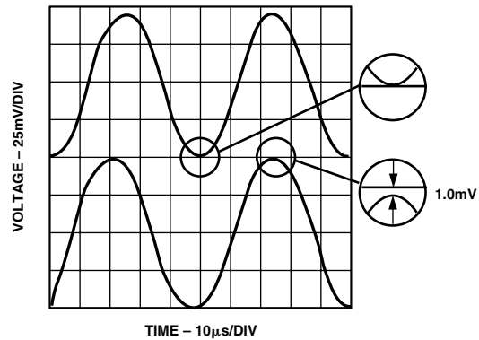
Figure 6. Rail-to-Rail Operation
