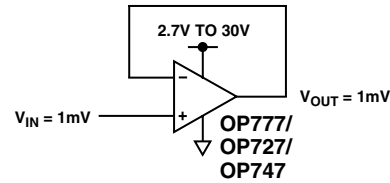
Figure 5. Follower Circuit
