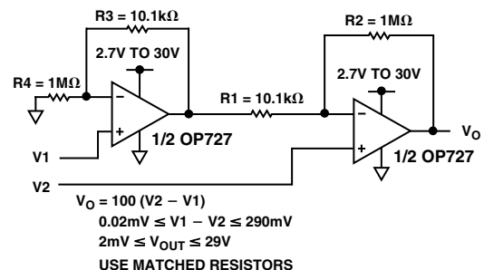
Figure 11. Single Supply Micropower Instrumentation Amplifier
