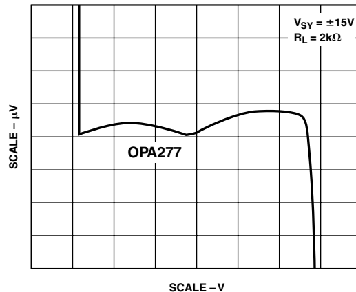
Figure 2. Gain Linearity
