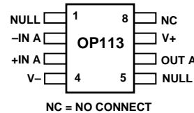
8-Lead Narrow-Body SO (S Suffix)
