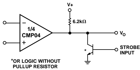
Figure 12. Output Strobing
