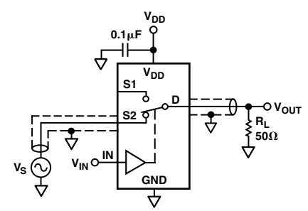
Test Circuit 8. Bandwidth
