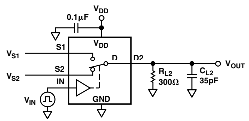
Test Circuit 5. Break-Before-Make Time Delay, t_D
