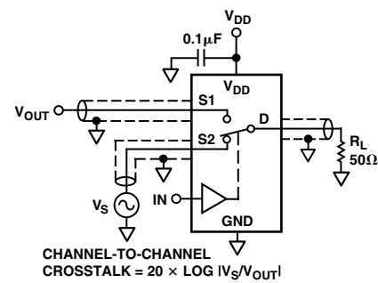
Test Circuit 7. Channel-to-Channel Crosstalk CHANNEL-TO-CHANNEL CROSSTALK = 20 \times \log |V_S/V_{OUT}|
