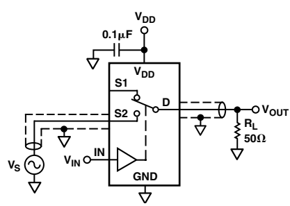
Test Circuit 6. Off Isolation
