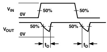
Test Circuit 5. Break-Before-Make Time Delay, t_D
