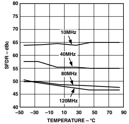
TPC 15. SFDR vs. Temperature, f_{DAC} = 300 MSPS @ 0 dBFS
