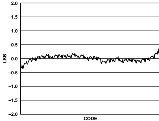
Figure 19. Integral Nonlinearity
