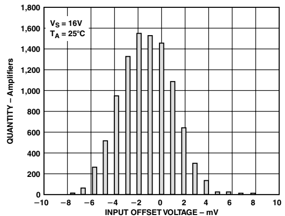
TPC 18. Input Offset Voltage Distribution
