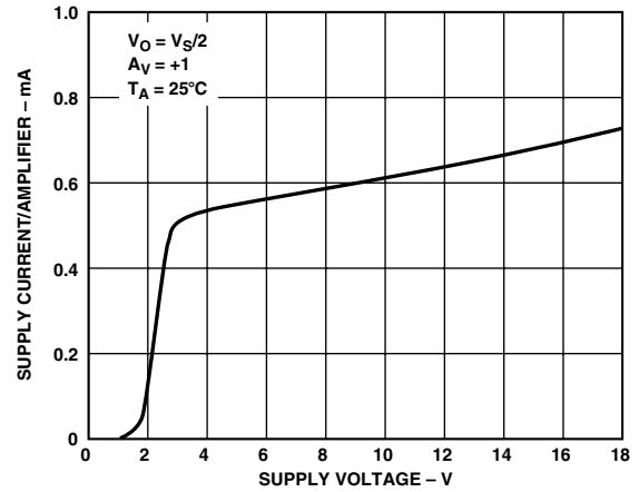
TPC 5. Supply Current/Amplifier vs. Supply Voltage
