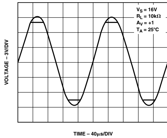
TPC 17. No Phase Reversal
