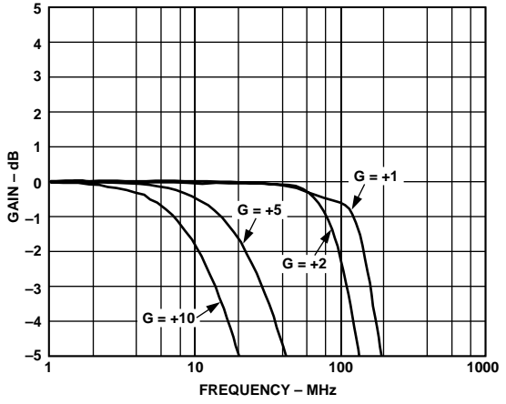
Figure 19. Large Signal Frequency Response, V_{OUT} = 2 \text{ V p-p}
