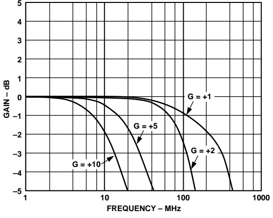
Figure 18. Small Signal Frequency Response, V_{OUT} = 0.2 \text{ V p-p}
