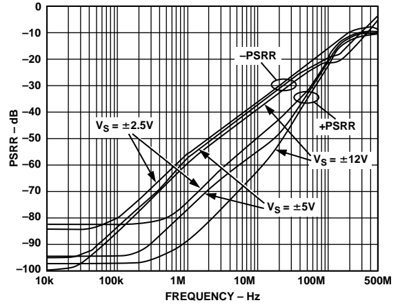
TPC 41. PSRR vs. Frequency and Supply Voltage. See Test Circuits 9 and 10.
