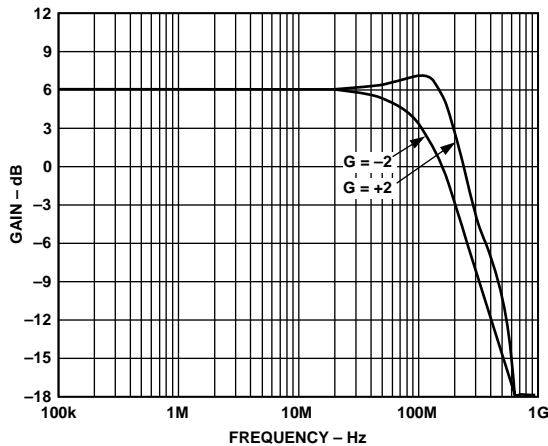
Figure 11. AC Response of Two Identically Compensated High-Speed Op Amps Configured for Gain of +2 and -2
