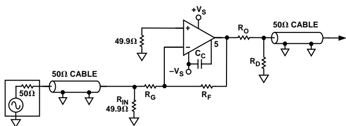
Test Circuit 3. Inverting Gain Test Circuit
