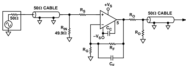
Test Circuit 1. Noninverting Gain Test Circuit
