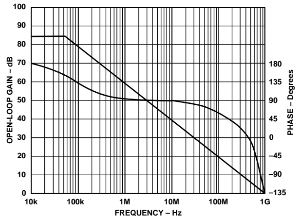
TPC 12. Open-Loop Gain and Phase vs. Frequency. R_G = 100\ \Omega , R_F = 1\ \text{k}\Omega , R_O = 976\ \Omega , R_D = 53.6 , C_C = 0\ \text{pF} . See Test Circuit 3.
