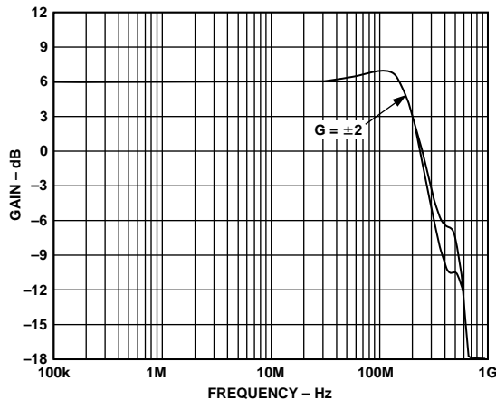
Figure 12. AC Response of Two Dissimilarly Compensated AD8021 Op Amps (Figure 11) Configured for Gain of +2 and -2. Note the Close Gain Match.
