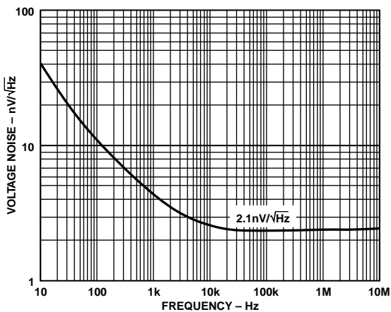
TPC 32. Input Voltage Noise vs. Frequency
