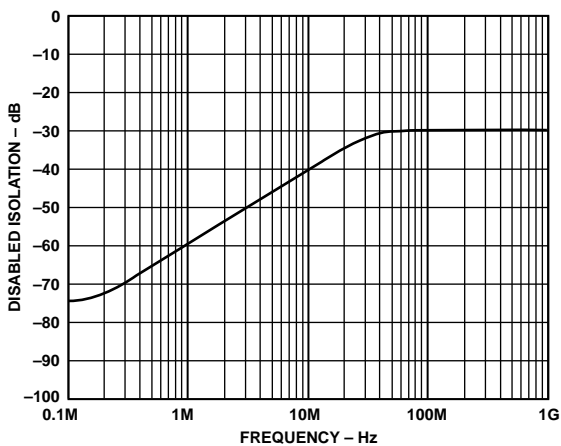
TPC 39. Input to Output Isolation, Chip Disabled. See Test Circuit 7.
