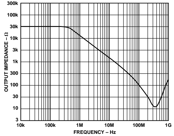
TPC 40. Output Impedance vs. Frequency, Chip Disabled. See Test Circuit 8.
