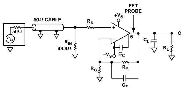
Test Circuit 2. Noninverting Gain Test Circuit with FET Probe
