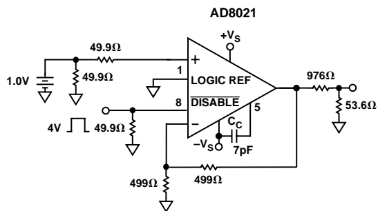
Test Circuit 6. Enable/Disable Test Circuit
