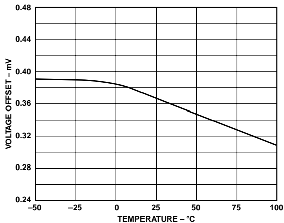
TPC 34. V_{OS} vs. Temperature
