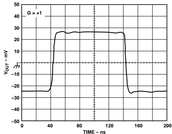
TPC 31. Small Signal Transient Response, V_O = 50 mV p-p. G = +1 . See Test Circuit 1.
