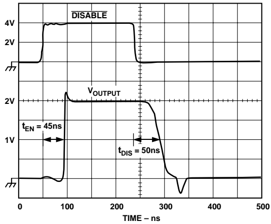
TPC 38. Enable ( t_{EN} )/Disable ( t_{DIS} ) Time vs. V_{OUT} . See Test Circuit 6.
