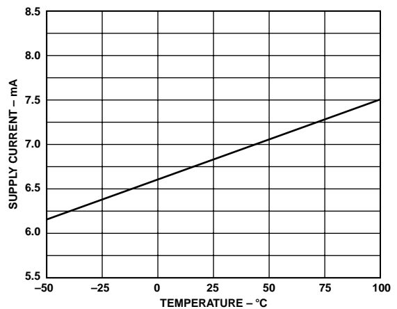
TPC 42. Quiescent Supply Current vs. Temperature
