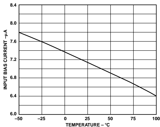
TPC 35. Input Bias Current vs. Temperature
