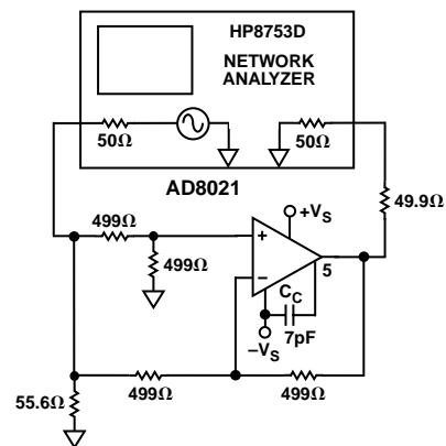
Test Circuit 4. CMRR Test Circuit
