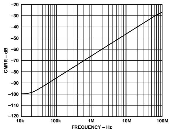
TPC 36. CMRR vs. Frequency. See Test Circuit 4.
