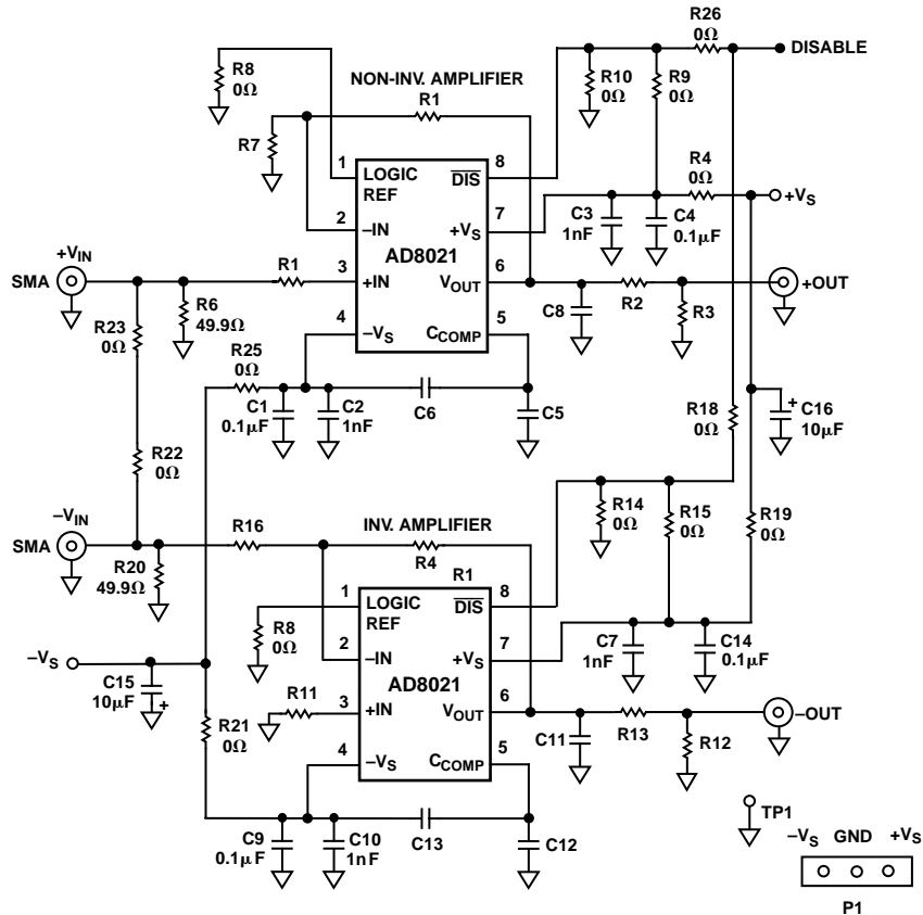
Figure 17. Schematic of AD8021 Evaluation Board
