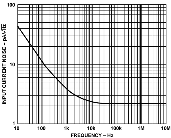
TPC 33. Input Current Noise vs. Frequency
