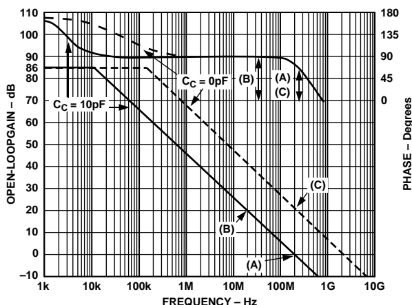
Figure 3. Simplified Diagram of AD8021 Open-Loop Gain and Phase Response
