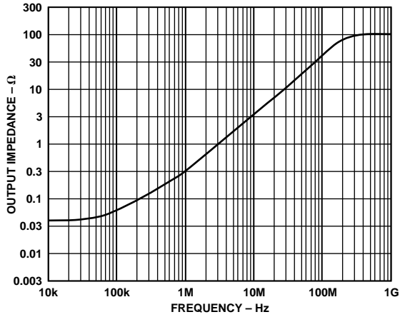
TPC 37. Output Impedance vs. Frequency, Chip Enabled. See Test Circuit 5.
