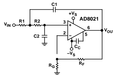
Figure 13. Schematic of a Second Order Low-Pass Active Filter
