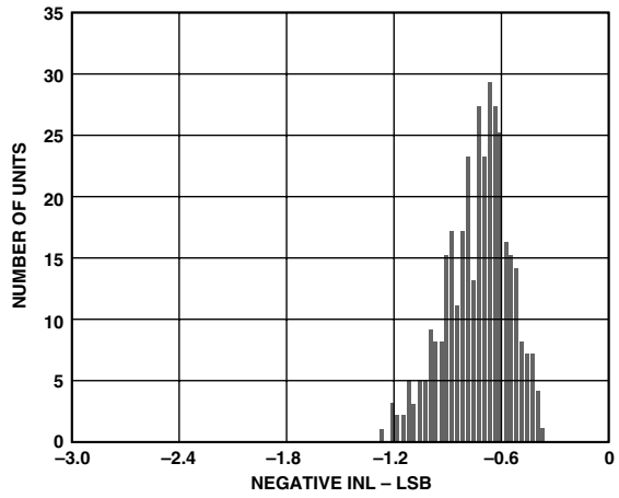
TPC 5. Typical Negative INL Distribution (350 Units)
