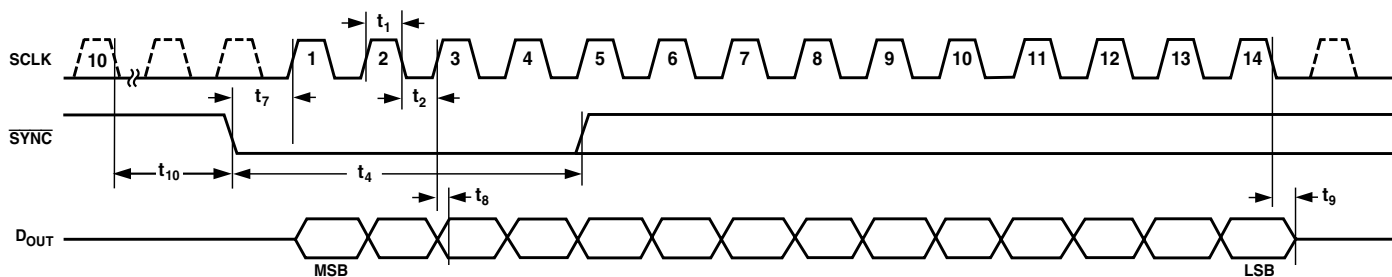
Figure 5. 14-Bit Read (Both Readback Modes)
