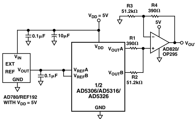
Figure 15. Coarse/Fine Adjustment
