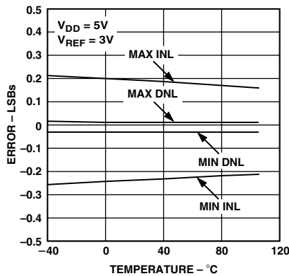
TPC 8. AD5306 INL Error and DNL Error vs. Temperature
