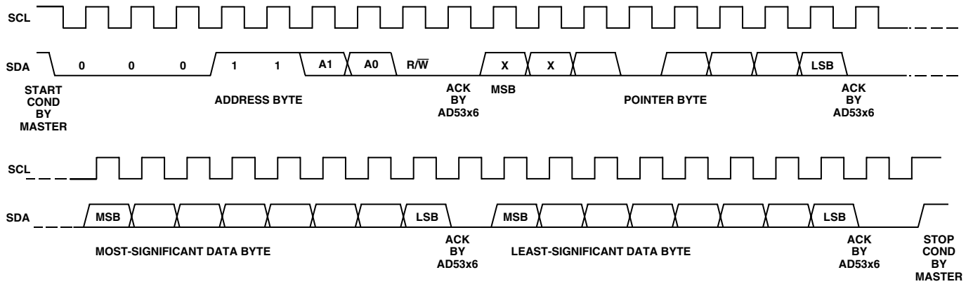
Figure 8. Write Sequence
