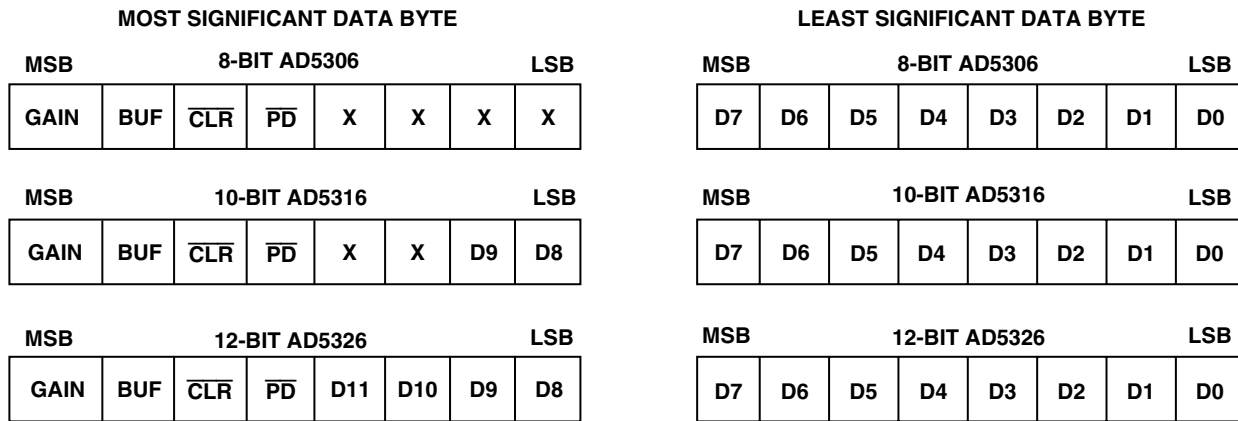
Figure 7. Data Formats for Write and Readback
