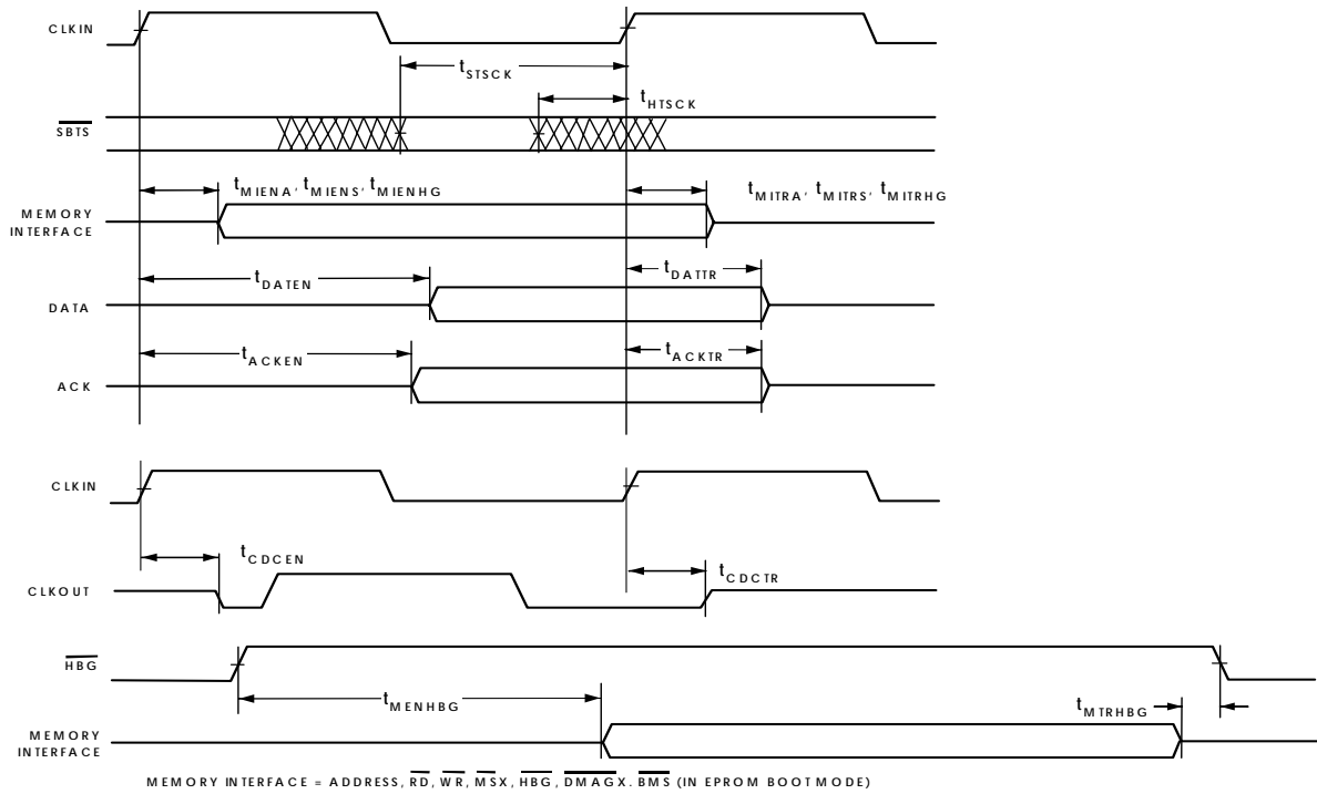
Figure 26. Three-State Timing
