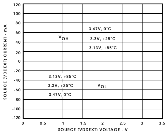
Figure 36. ADSP-21161N Typical Drive
