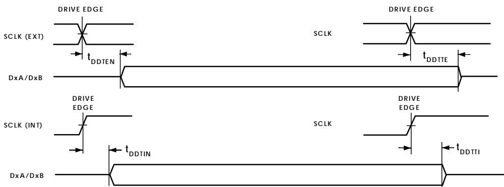
Figure 31. Serial Ports
