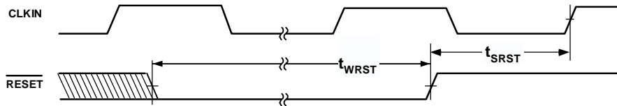
Figure 16. Reset
