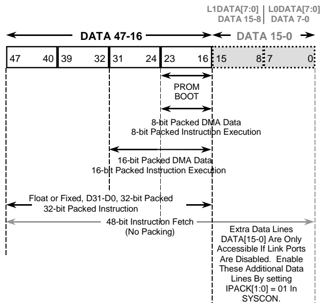
Figure 3. ADSP-21161N External Data Alignment Options
