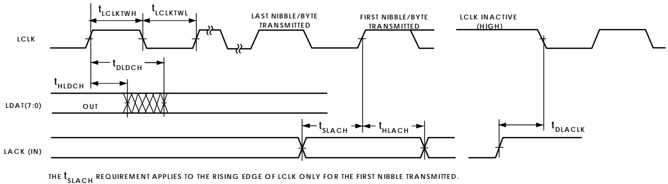
Figure 30. Link Ports—Transmit
