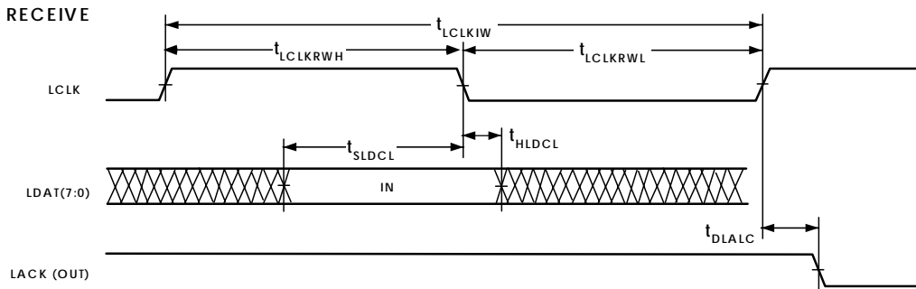
Figure 29. Link Ports—Receive
