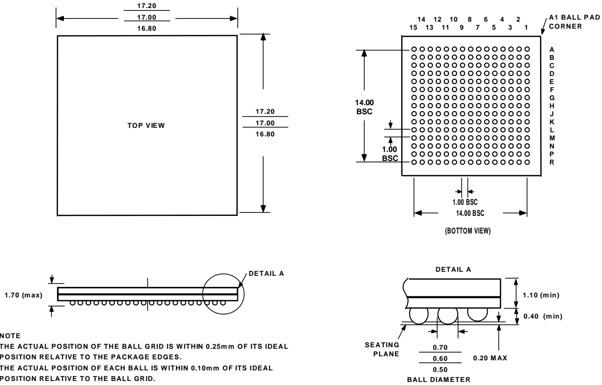
Figure 44. Package Dimensions Metric 17mm × 17mm, 225 ball MBGA
