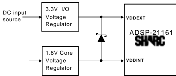
Figure 13. Dual Voltage Schottky Diode
