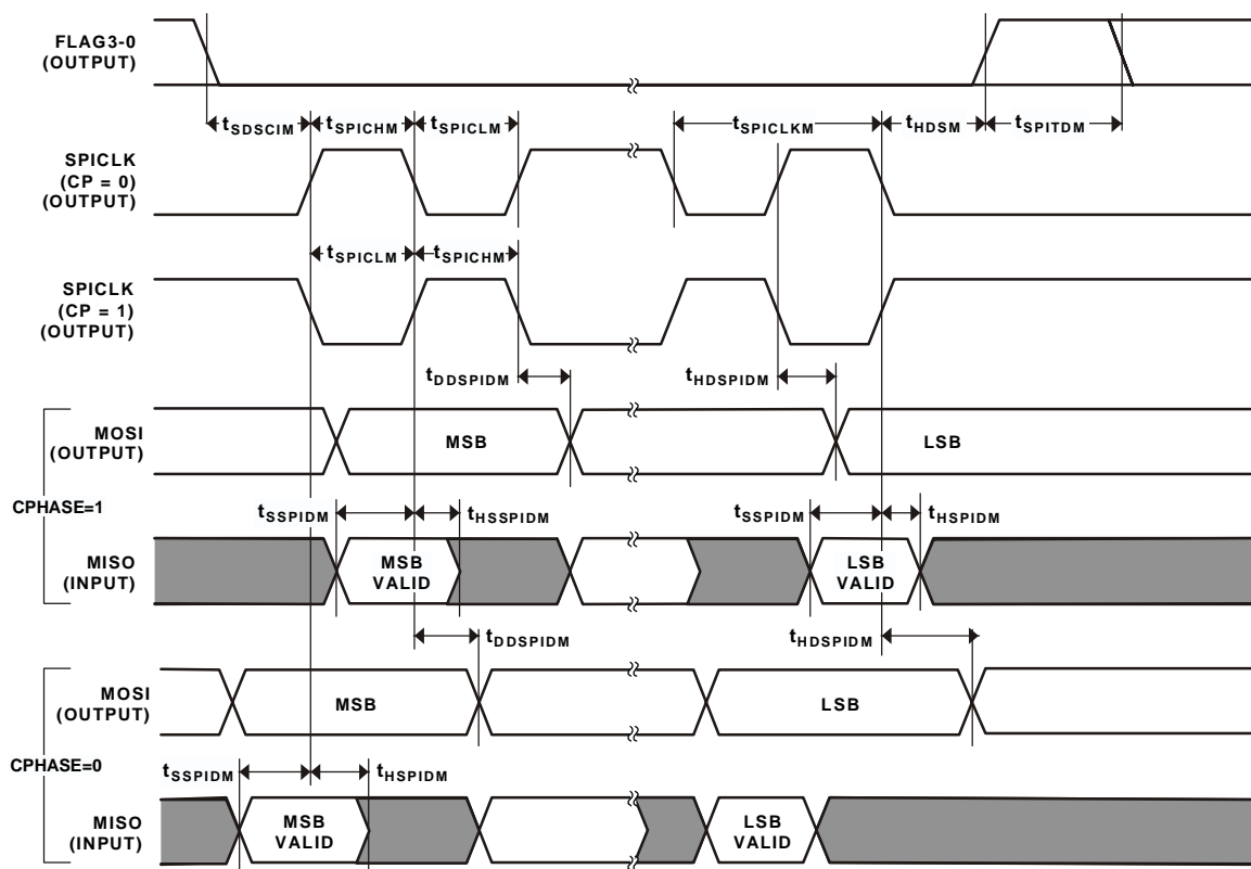
Figure 33. SPI Master Timing
