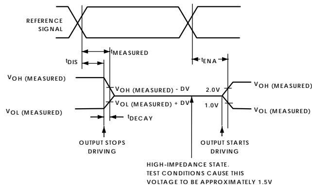
Figure 37. Output Enable/Disable
