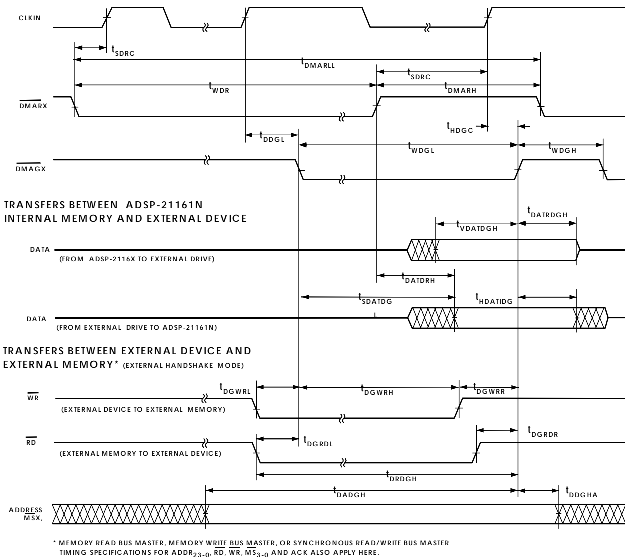
Figure 27. DMA Handshake Timing
