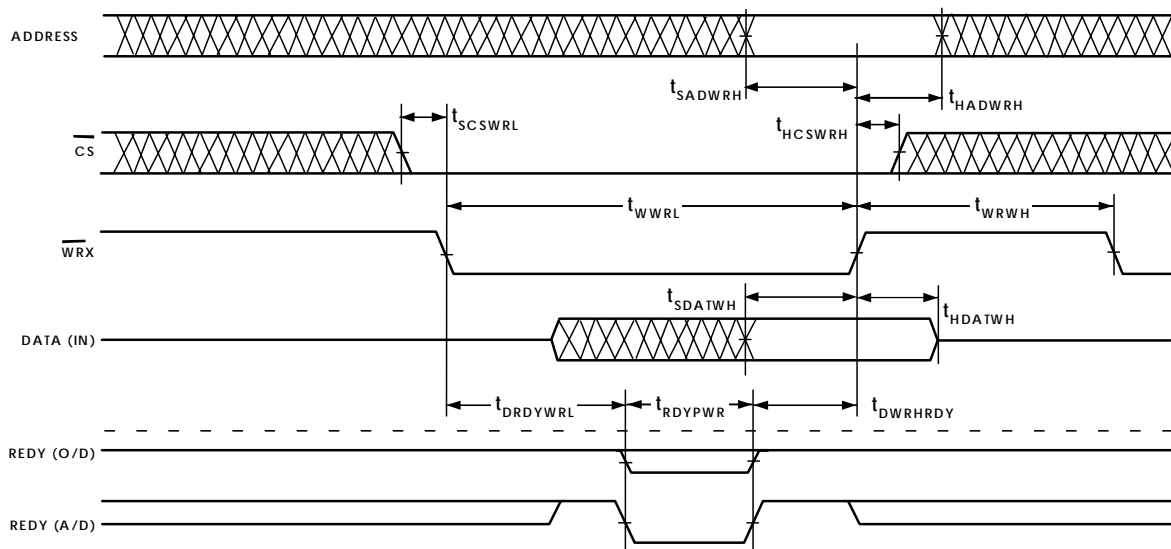
Figure 25. Asynchronous Read/Write--Host to ADSP-21161N
