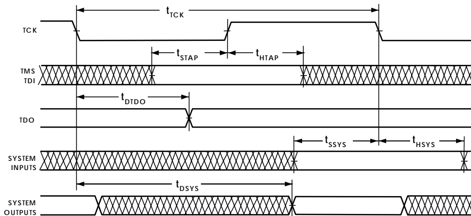
Figure 35. IEEE 11499.1 JTAG Test Access Port
