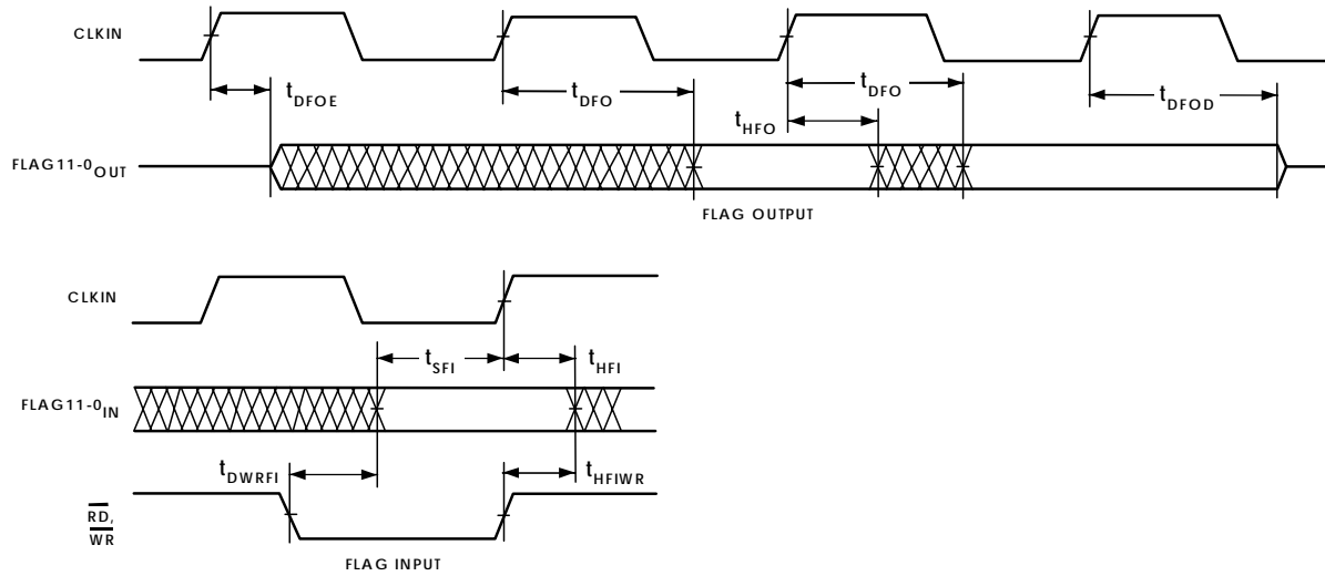
Figure 19. Flags
