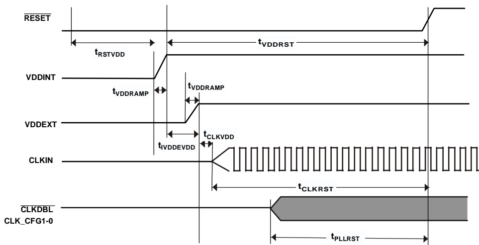
Figure 11. Power Up Sequencing for Revisions 0.3, 1.0, and 1.1
