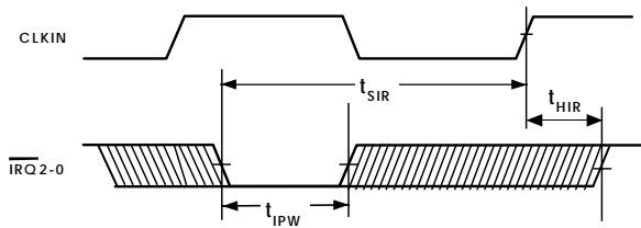
Figure 17. Interrupts
