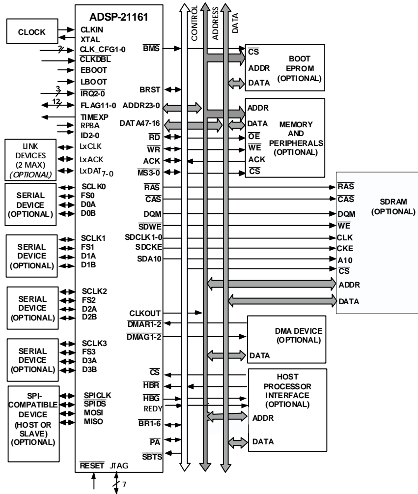
Figure 1. ADSP-21161N System
