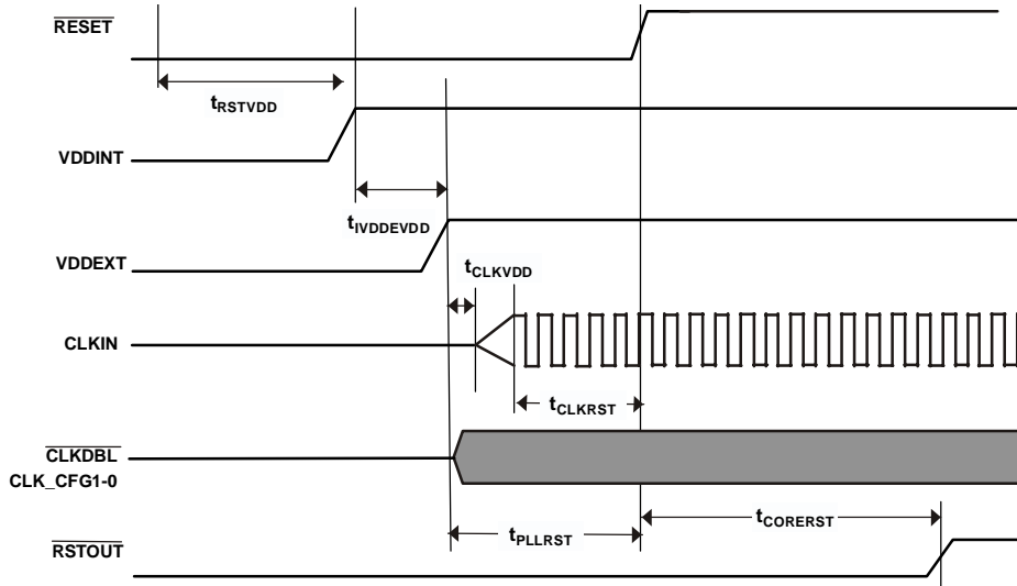
Figure 12. Power Up Sequencing for 1.2
