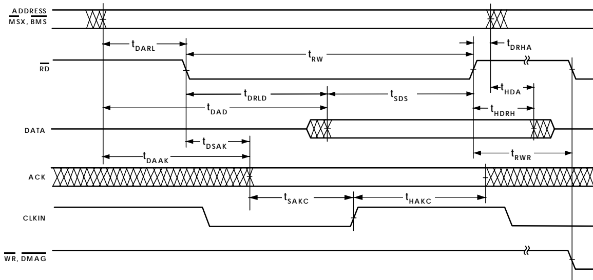
Figure 20. Memory Read--Bus Master
