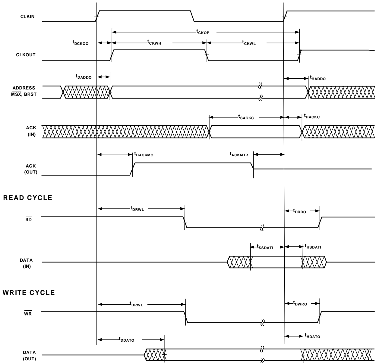
Figure 22. Synchronous Read/Write--Bus Master
