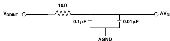
Figure 5. Analog Power ( V_{DD} ) Filter Circuit
