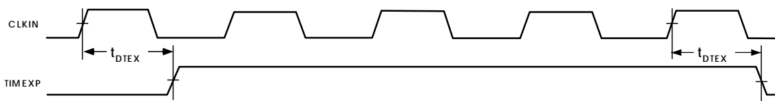
Figure 18. Timer
