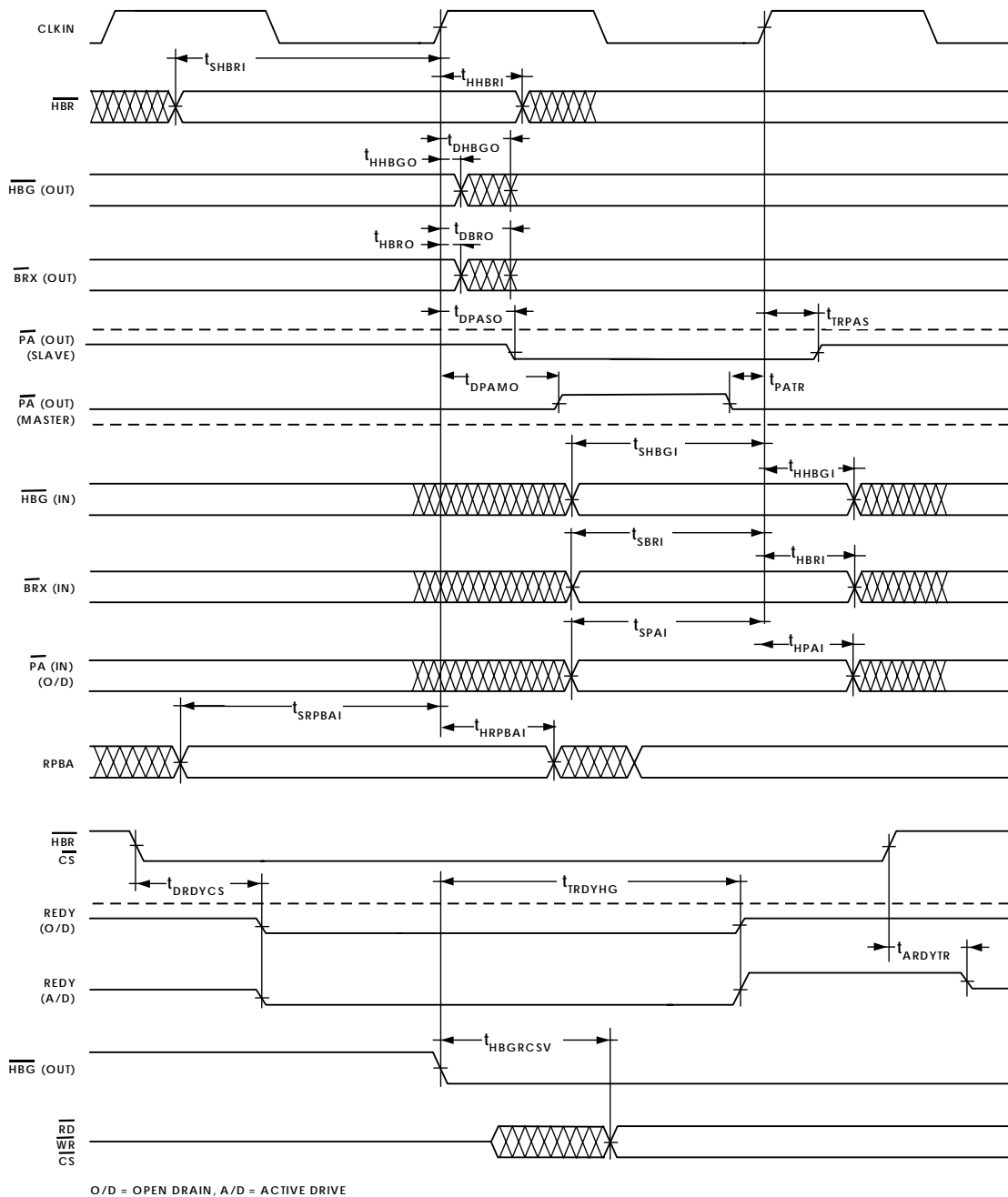
Figure 24. Multiprocessor Bus Request and Host Bus Request
