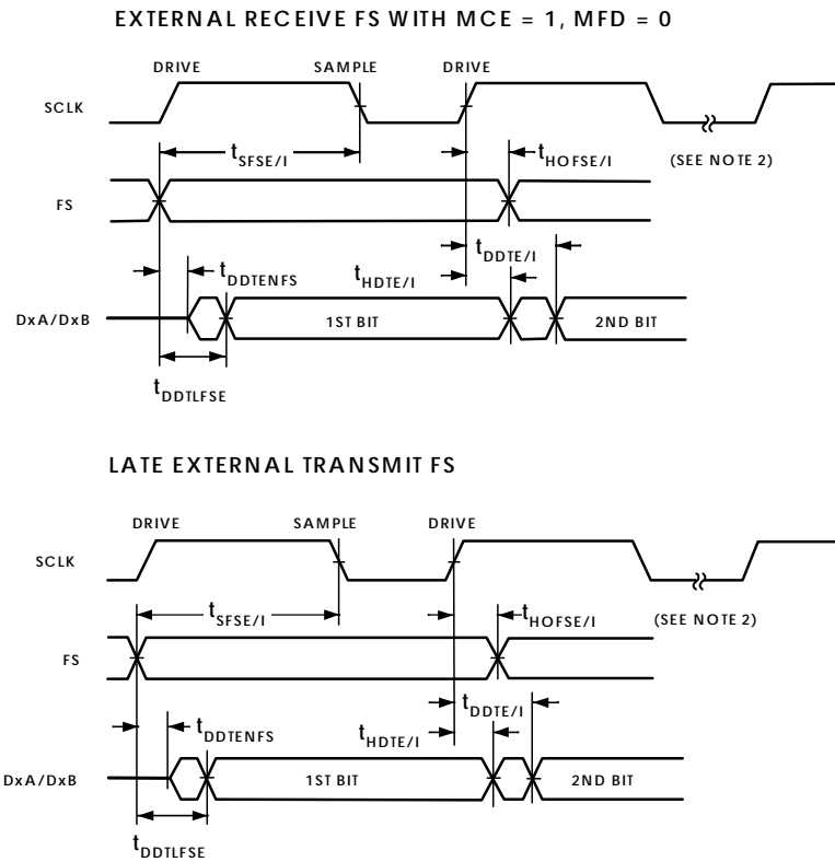
Figure 32. External Late Frame Sync
