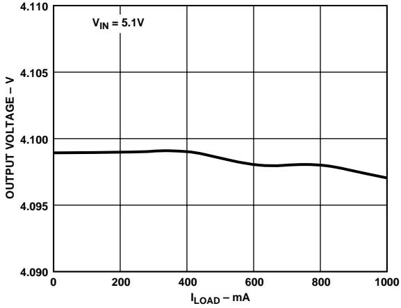
Figure 2. V_{OUT} vs. I_{LOAD} ( V_{IN} = 5.1 V )*
