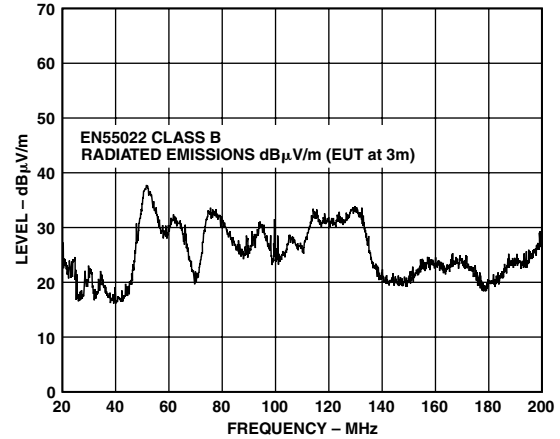
Figure 17. Radiated Emissions Plot
