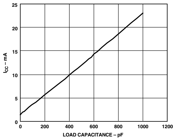
TPC 9. Supply Current vs. Load Capacitance ( R_L = \infty )
