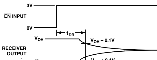
Figure 5. Receiver Disable Timing
