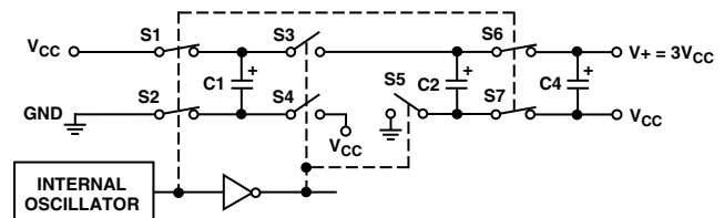
Figure 1. Charge Pump Voltage Tripler
