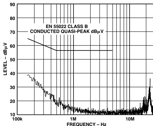
Figure 15. Conducted Emissions Plot
