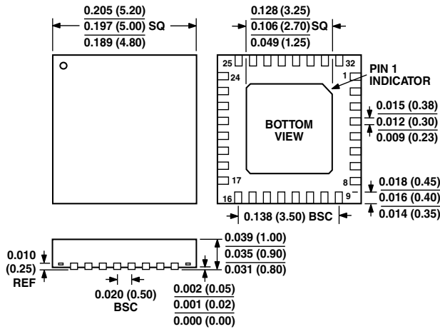
32-Lead LFCSP (CP-32)
