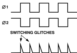
Figure 14. Switching Glitches
