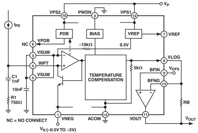
Figure 15. Using the Buffer to Invert the Polarity of the Slope
