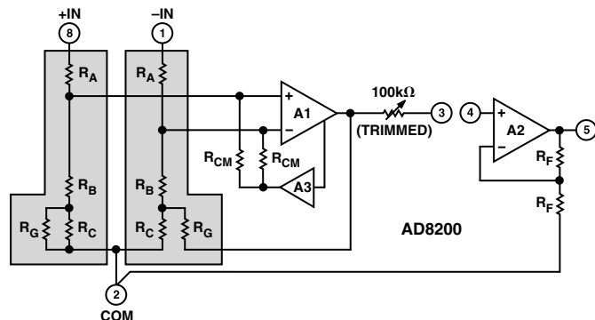
Figure 3. Simplified Schematic
