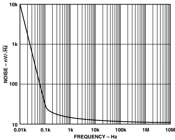
TPC 20. Noise vs. Frequency
