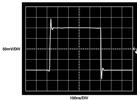
TPC 24. Small Signal Pulse Response, V_S = \pm 12 V , R_L = 600 \Omega
