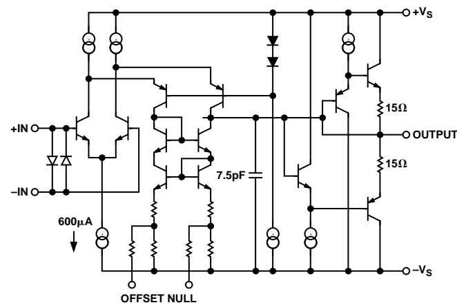
Figure 35. Simplified Schematic
