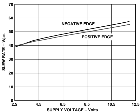
Figure 8. Slew Rate vs. Supply Voltage, V_S = \pm 12\text{ V} , G = 2
