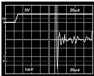
Figure 12c. Turn-On Settling
