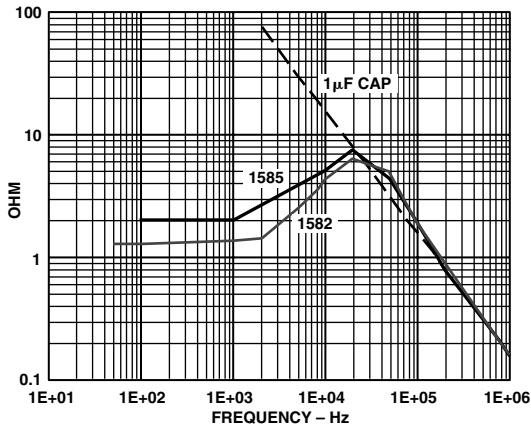
Figure 8b. Output Impedance vs. Frequency
